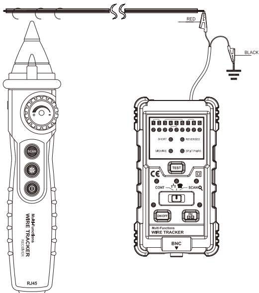
Other metal cable line diagram
